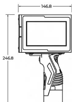
R10H Handheld TIJ
