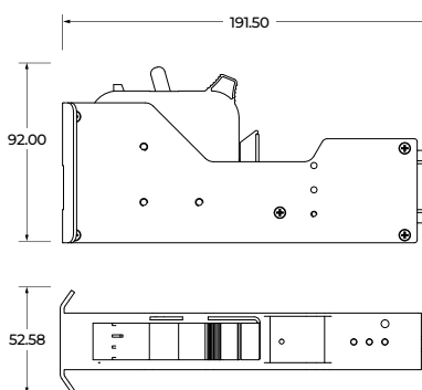
PROe Printhead
