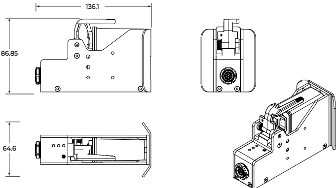
REACH Printhead
